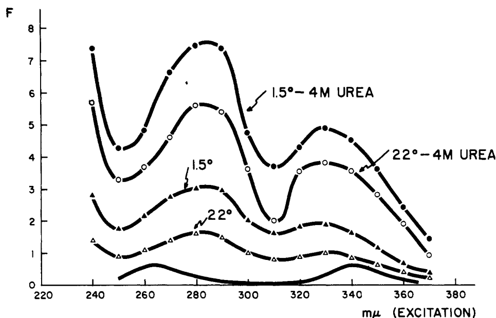
FIG. 10.—The effect of cooling and 4 M urea on the fluorescence excitation spectrum of the liver alcohol dehydrogenase-DPNH complex. The concentration of the enzyme was 4 \times 10^{-6} M and the concentration of the coenzyme 6 \times 10^{-6} M. The solid points were obtained at 1.5° in the presence of 4 M urea and the open circles at 22° in the presence of 4 M urea. The solid triangles were obtained at 1.5° with no urea and the open triangles at 22° with no urea. The solid line represents the coenzyme alone. The measurements were obtained in the presence of 0.1 M phosphate buffer at pH 7.4.
